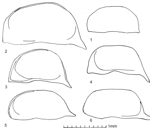
Fig. 1: Baraolt Carpathocandona species flock – female LV: 1. C. aff. bimucronata KLIE, 2. C. loerenthei n. sp., 3. C. aff. loerenthei n. sp., 4. C. krezoii n. sp., 5. C. brasovica n. sp., 6. C. aff. krezoii n. sp.
